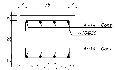
SEC B-B H Scale 1:25 V Scale 1:25
