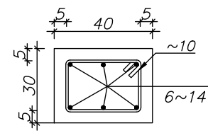
SEC 1-1 Scale 1:20
