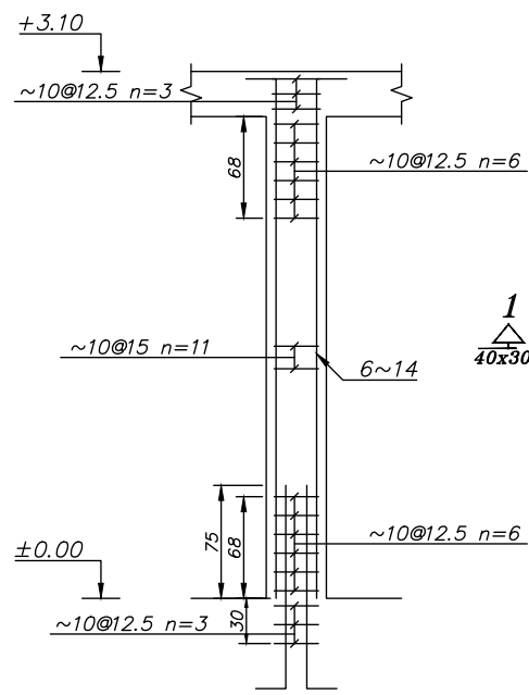
C-1 No.=14 Scale 1:50
