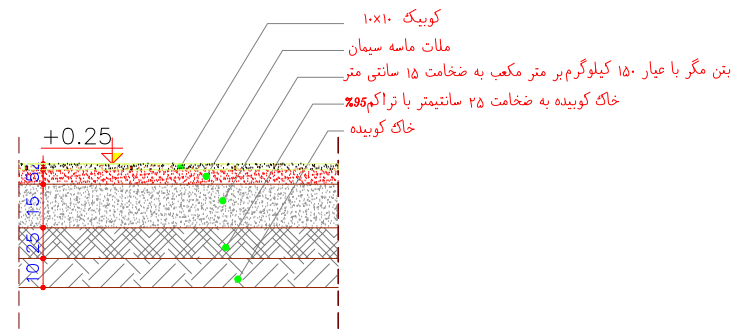
DETAIL 50
