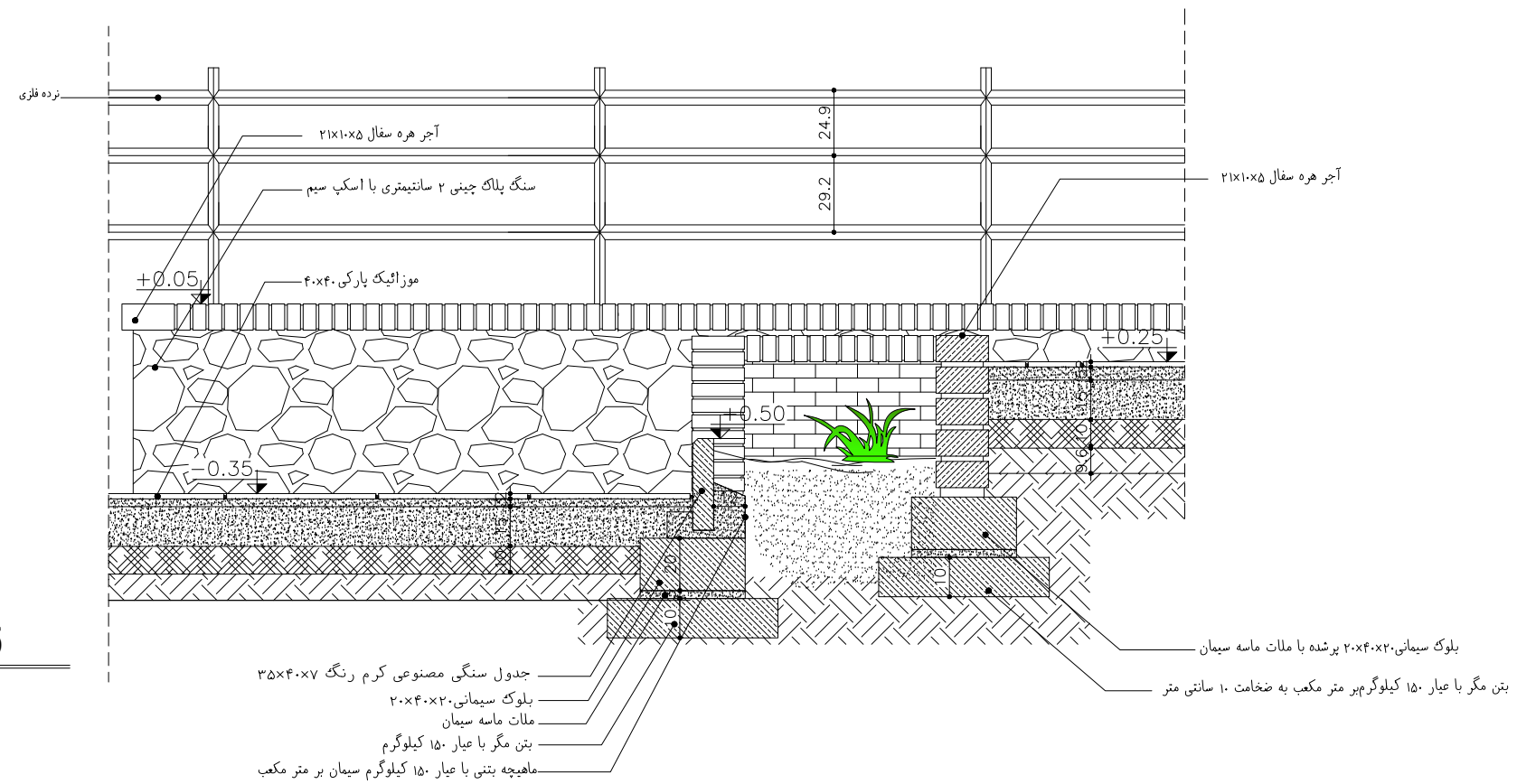
DETAIL 45 Sc - 1:20
