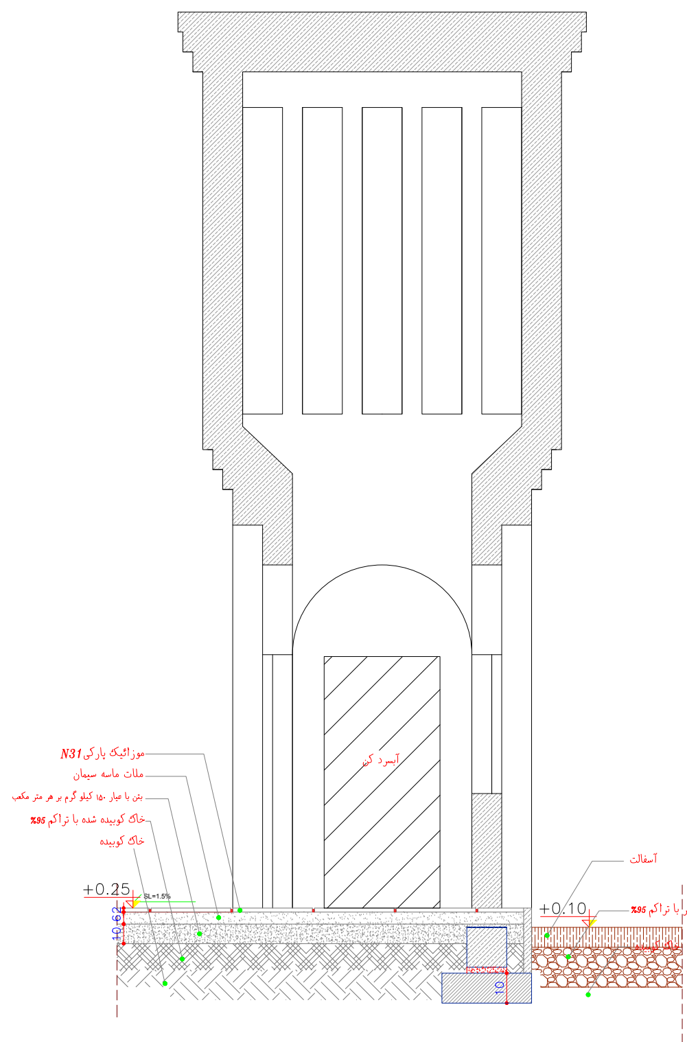
DETAIL 41 Sc - 1:20
