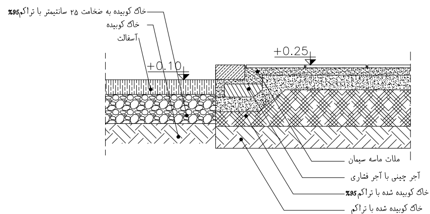
DETAIL 35 Sc - 1:20
