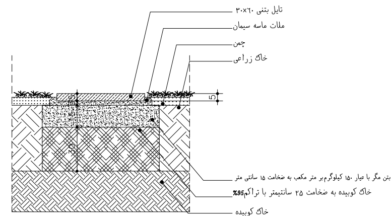
DETAIL 34 Sc - 1:20
