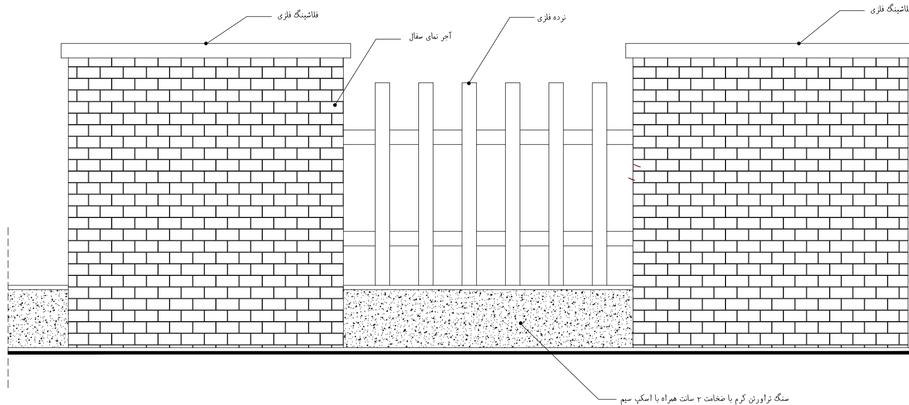
DETAIL 33 Sc - 1:20
