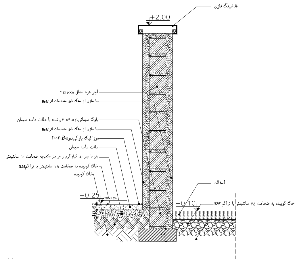
DETAIL 33 Sc - 1:20
