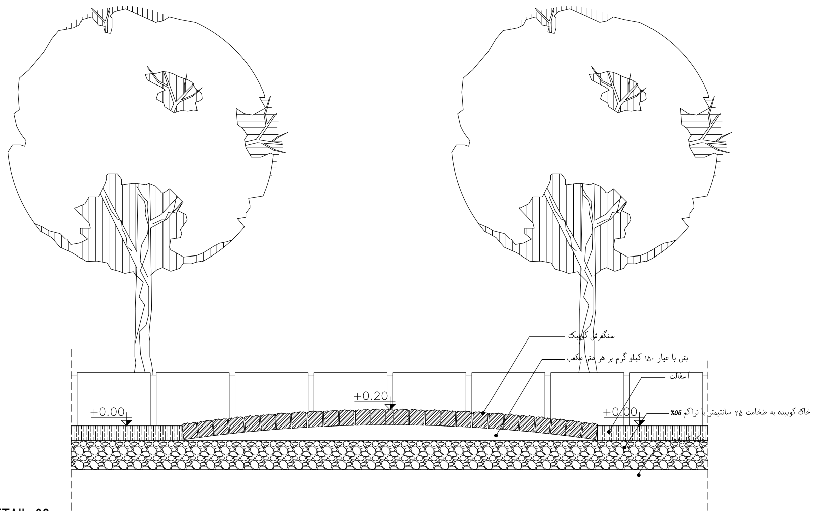
DETAIL 32 Sc - 1:20
